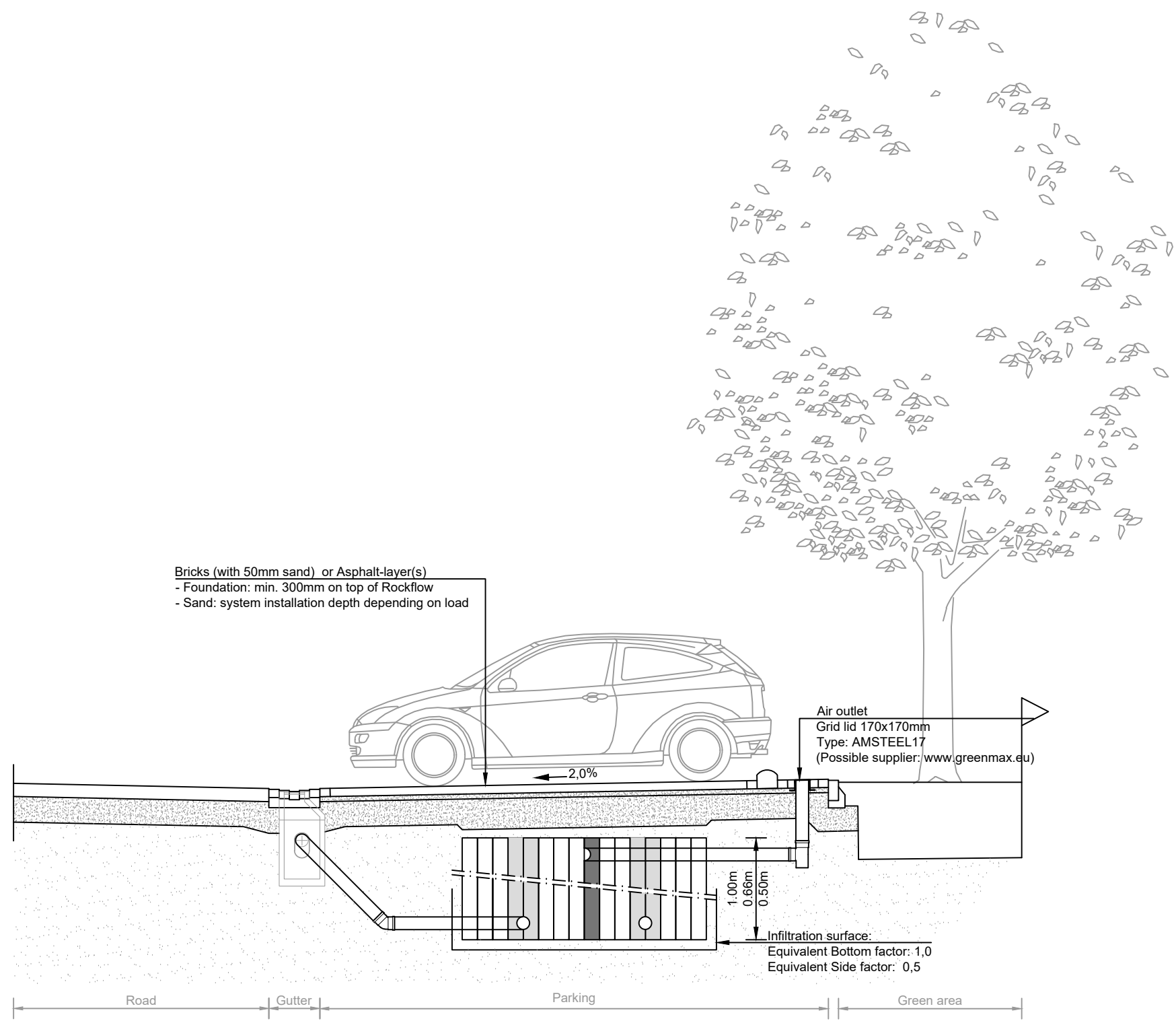
Cross section Water buffer Element height: 1,0m Scale 1:50
