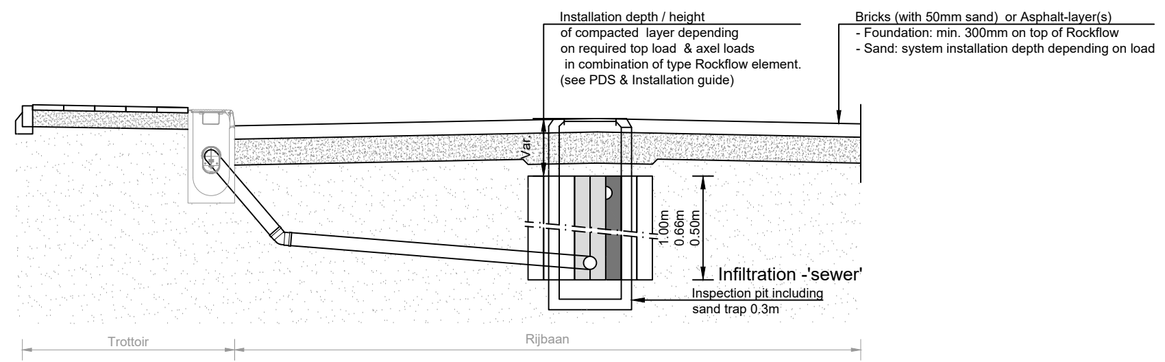
Cross section Line infiltration with pit Elements with different heights Scale 1:50
